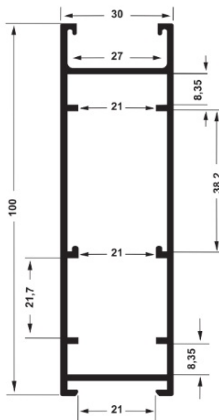
AL-3001 1,167 Kg/m
