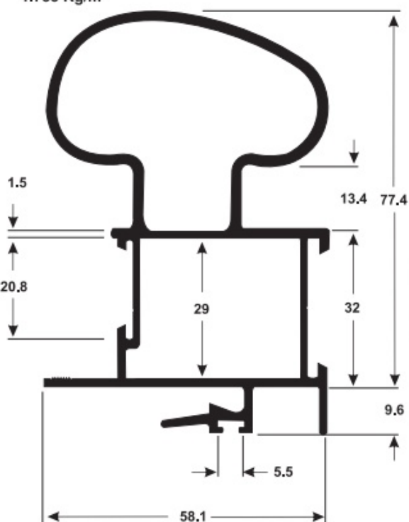
LG-021 1.733 Kg/m
