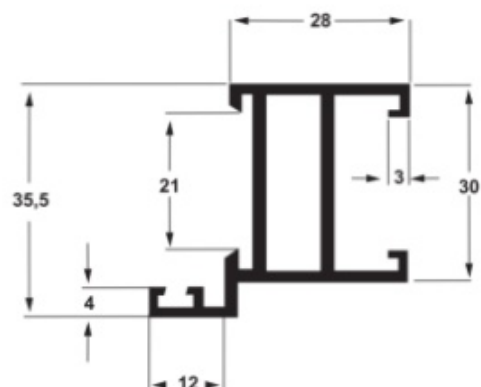
AL-3001 1,167 Kg/m
