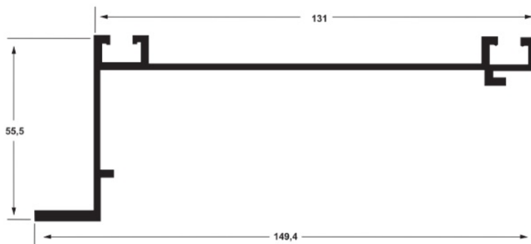
TP 6.00 - 8,400 Barra
