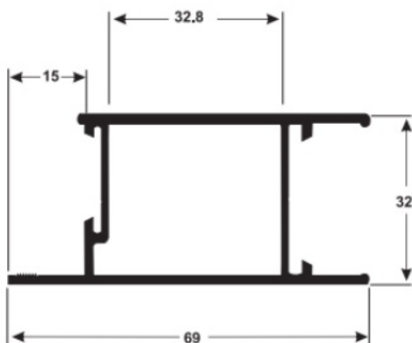
LG-021 1.733 Kg/m
